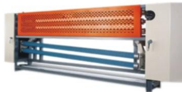
红外光电对中 Infrared photoelectric centering
