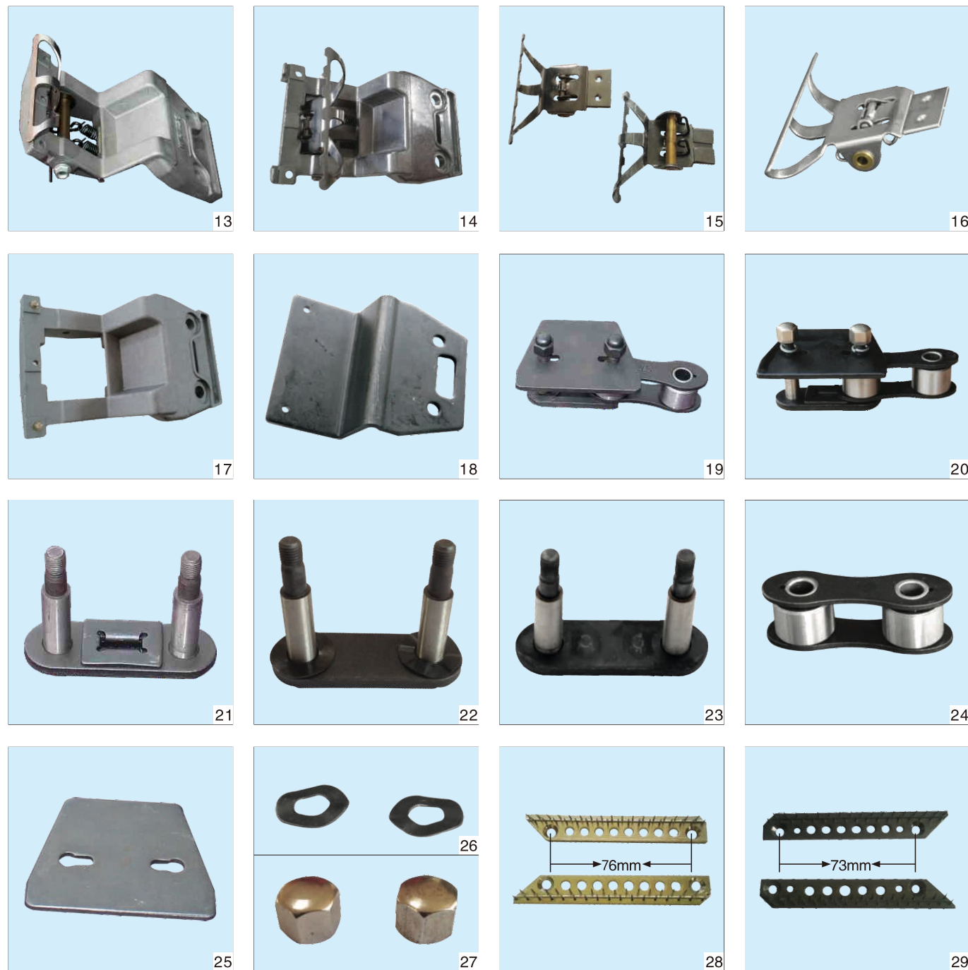
MFG-030 Pin Clip, Clip, pin holder, chain, pin plate Pitch: 50.8mm
