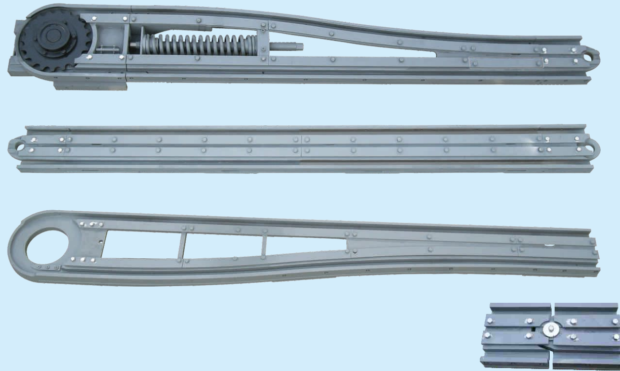
MFG-530 cast iron track
