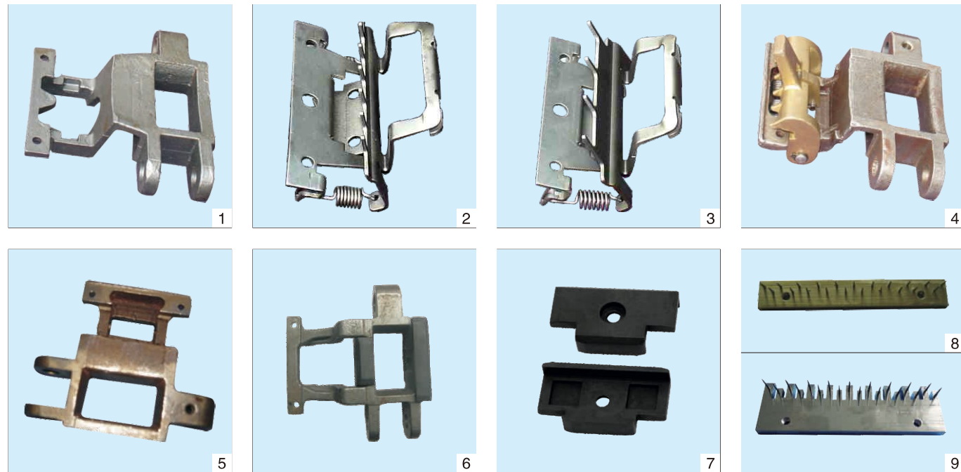
MFG-071 Vertical chain, pin holder, pin plate Pitch: 62.5mm
