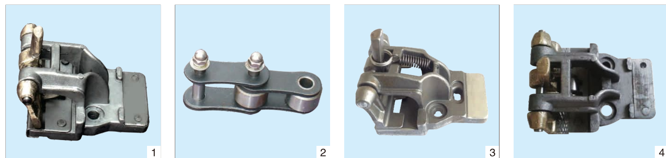
MFG-080 Clip, chain, pin holder Pitch: 38.1mm
